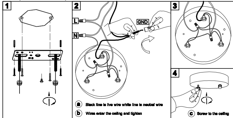
Wire Connection Diagram:
