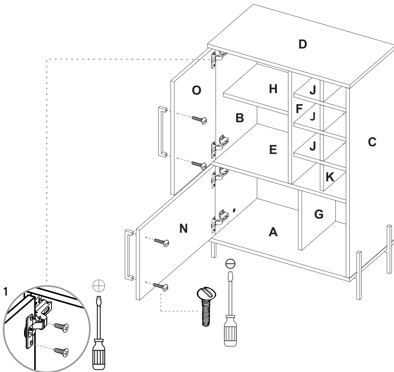
Hinge adjustment
