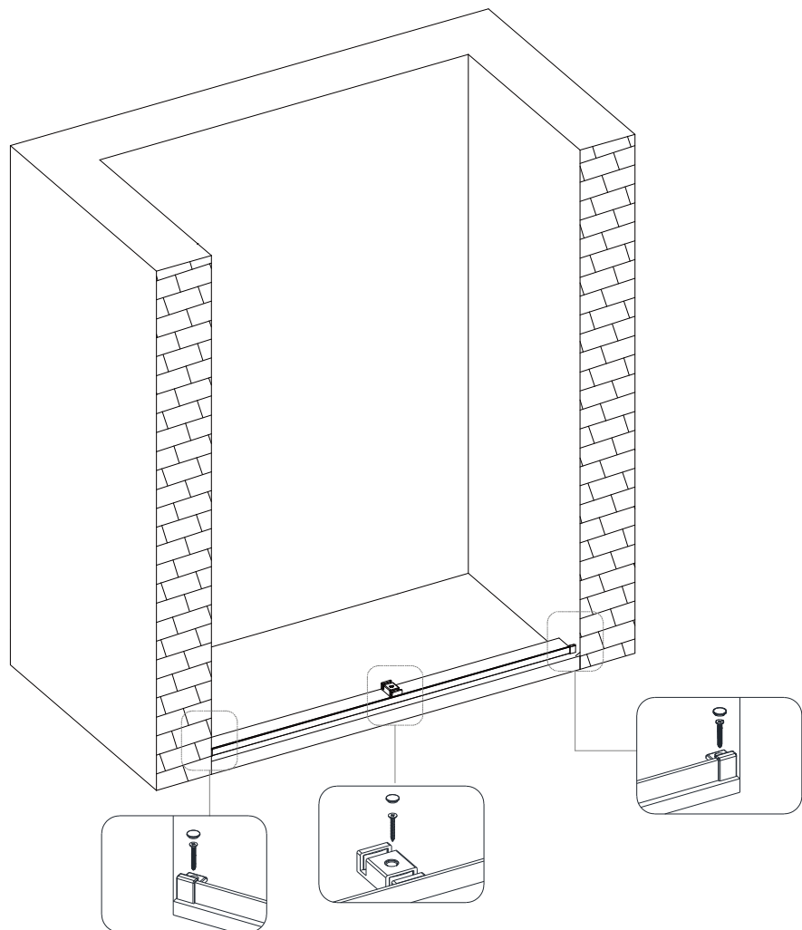
Lower Water Stop Bar Fixing Parts
