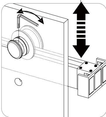
Debugging Guidelines for Door Glass.
