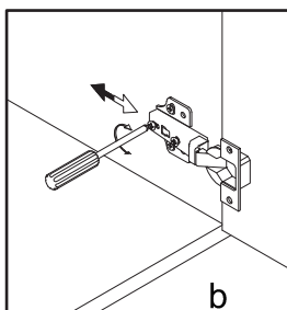
Door adjustment diagram :
