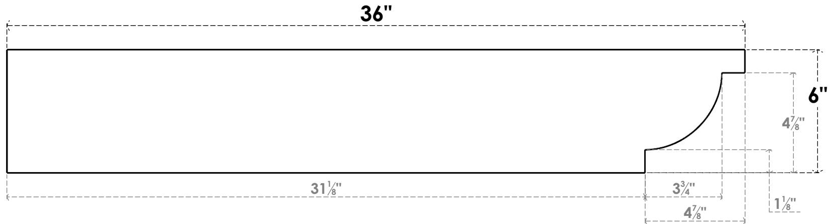
SIDE PROFILE
