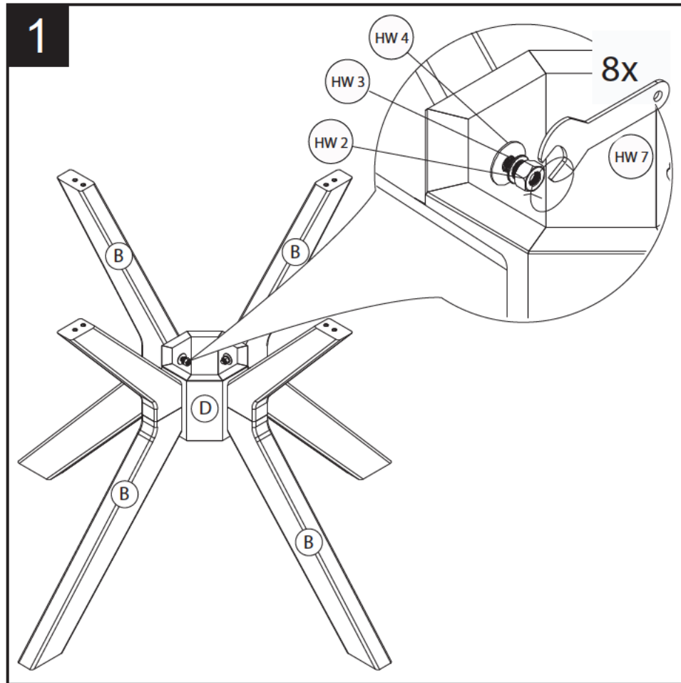
Step 1 Assemble the leg and pedestal.
