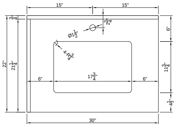
TOP VIEW OF VANITY CABINET
