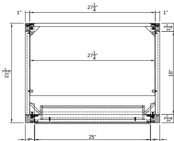
TOP VIEW OF VANITY CABINET
