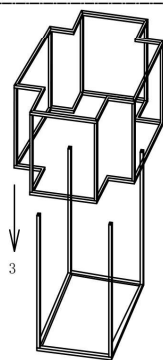
Shelf (C) ×1
