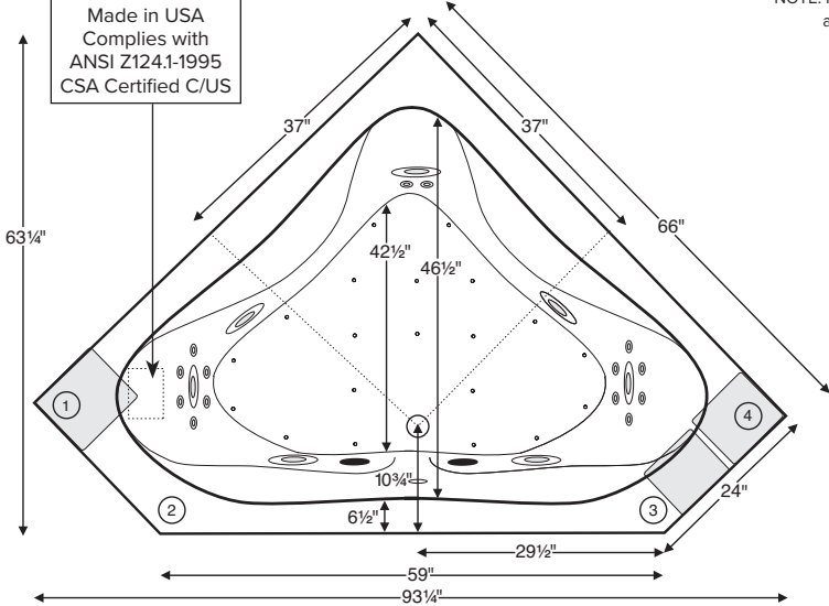
Numbered areas on tub deck represent possible locations to install cleaning systems, faucets and other fixtures.
