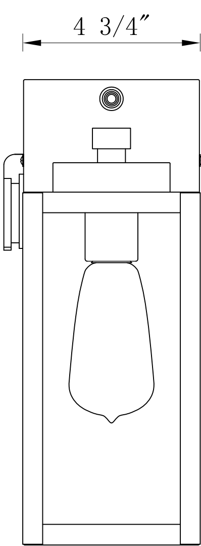
FRONT VIEW
