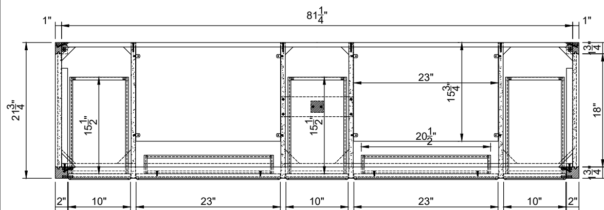
TOP VIEW OF VANITY CABINET
