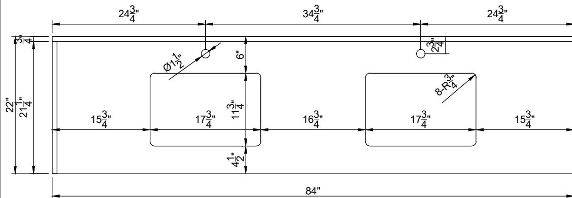
TOP VIEW OF VANITY CABINET
