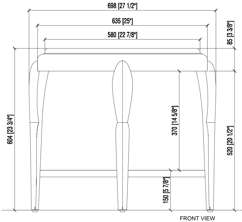
TA50294 27-1/2" x 27-1/2" x 23-3/4" HT
