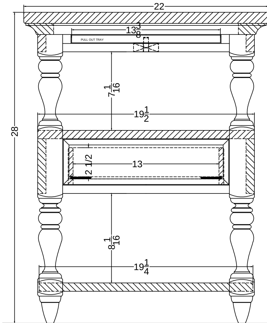
Nightstand 22"x 17"x 28" HT
