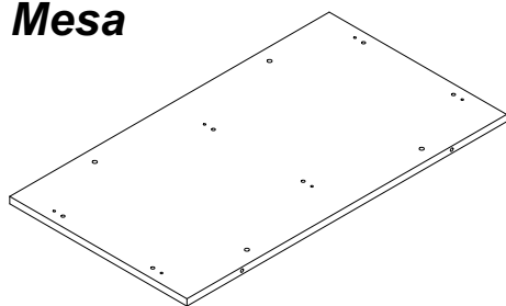
1 (914x507x18mm) X 1
