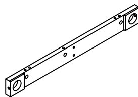
3 (740x75x27mm) X 2
