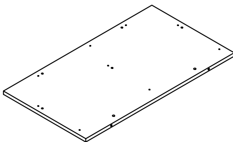
2 (914x506x18mm) X 2
