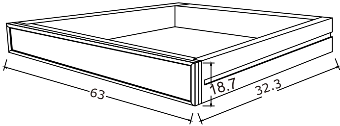
DRAWER DESIGN
