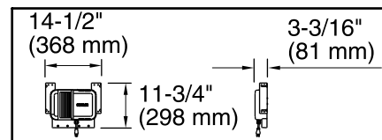
Control Amplifier
