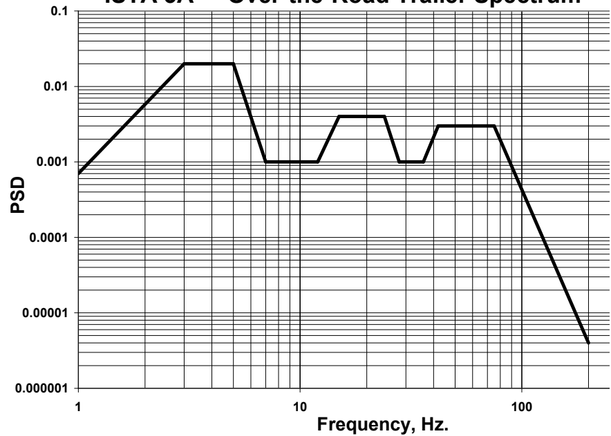
ISTA 3A - Over-the-Road Trailer Spectrum
