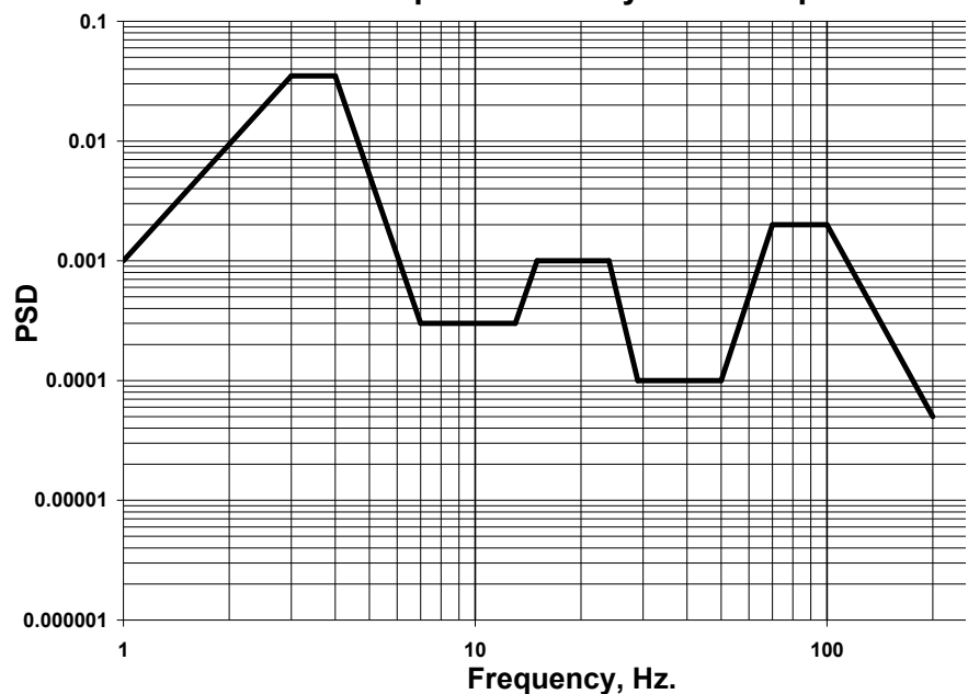
ISTA 3A - Pick-up and Delivery Vehicle Spectrum
