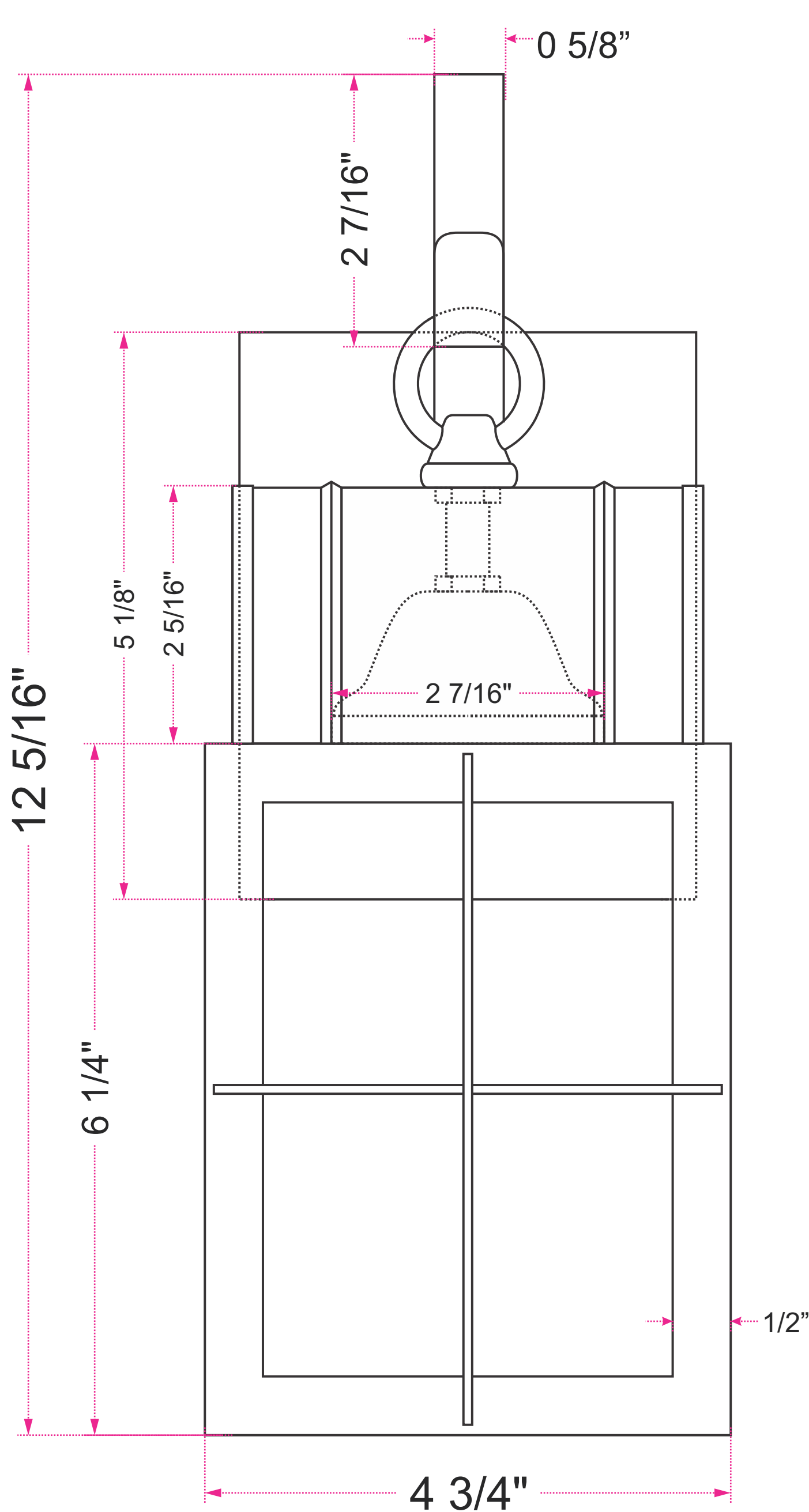
Front View
