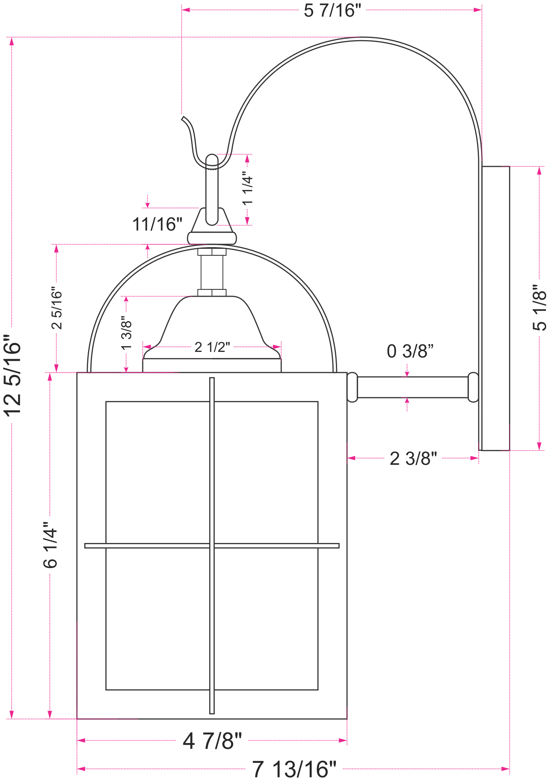
Side View
