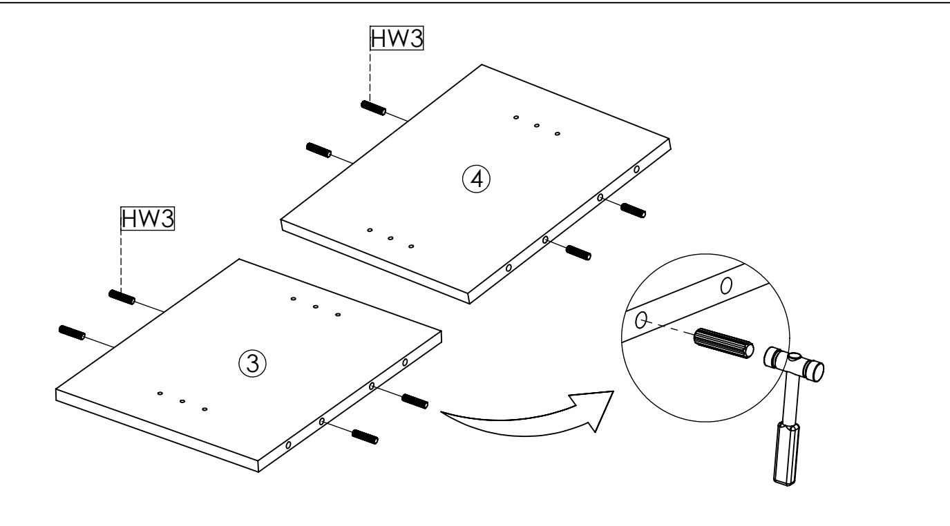
STEP3: Insert Wooden Dowel (HW3) into Left Center Panel (3) and Right Center Panel (4)
