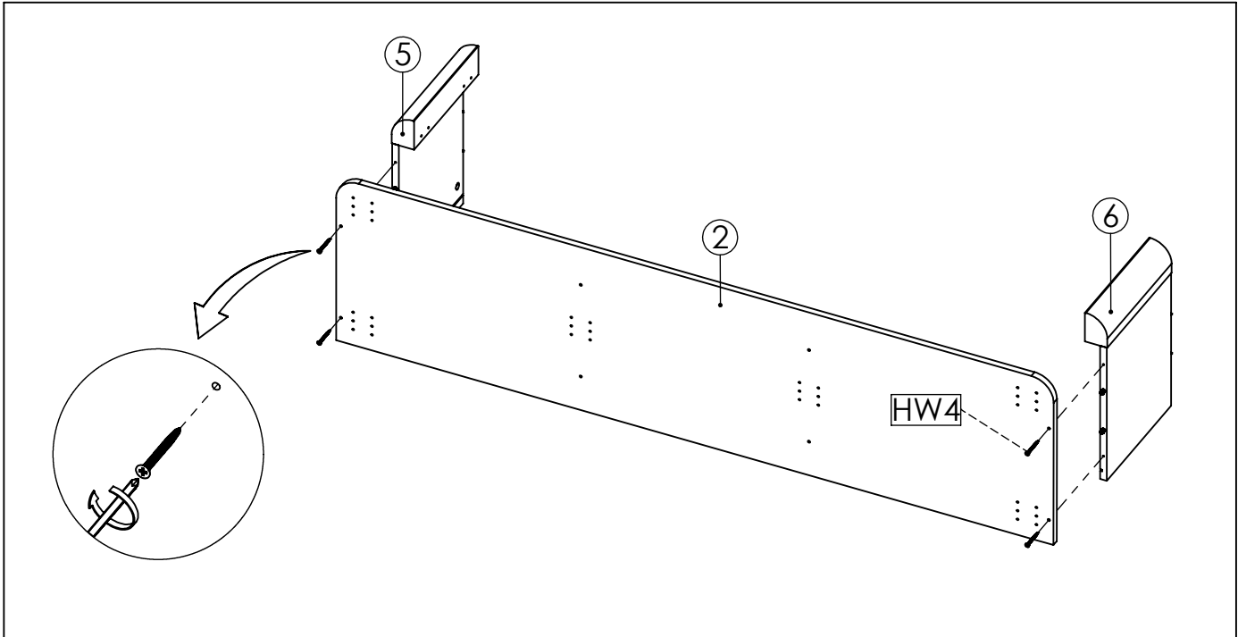
STEP2: Attach Left Side Panel (5) and Right Side Panel (6) into Bottom Panel (2), Next secure with Screw M6 x 50 (HW4) and tighten it using Screwdriver.
