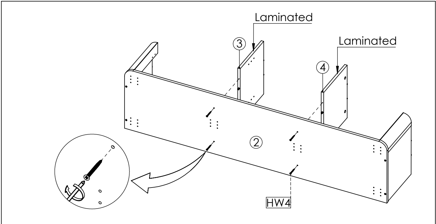
STEP4: Attach Left Center Panel (3) and Right Center Panel (4) into Bottom Panel (2), Next secure with Screw M6 x 50 (HW4) and tighten it using Screwdriver.
