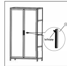
Install cabinet door handle: Tear off the handle adhesive diaphragm and stick the handle to the appropriate height position on the vertical strip of the cabinet door.
