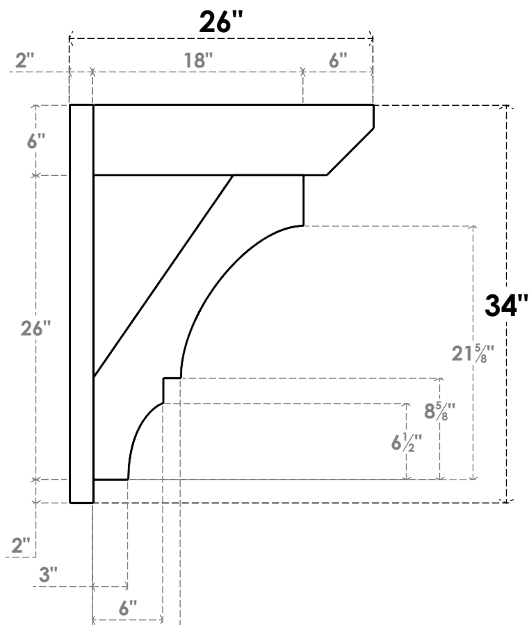
SIDE PROFILE
