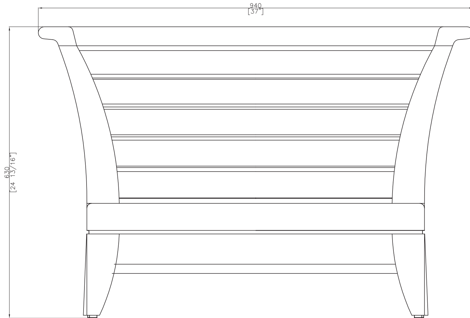
FRONT VIEW
