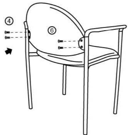
3 Back Joint
