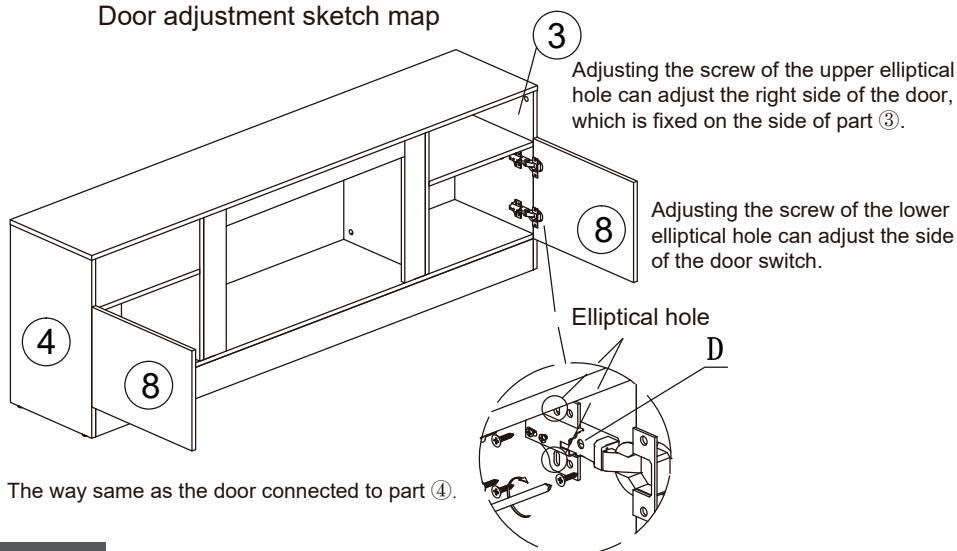
Door adjustment sketch map
