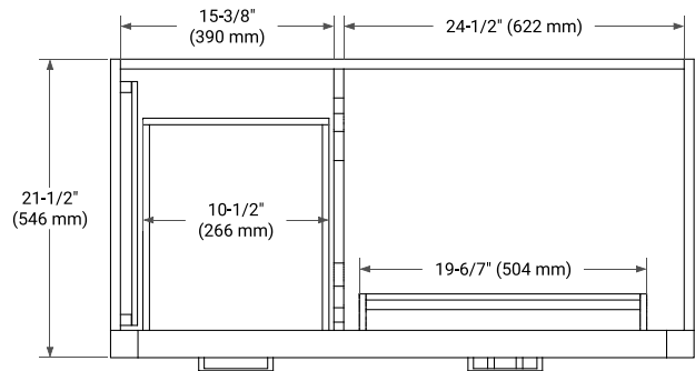
PLAN VIEW
