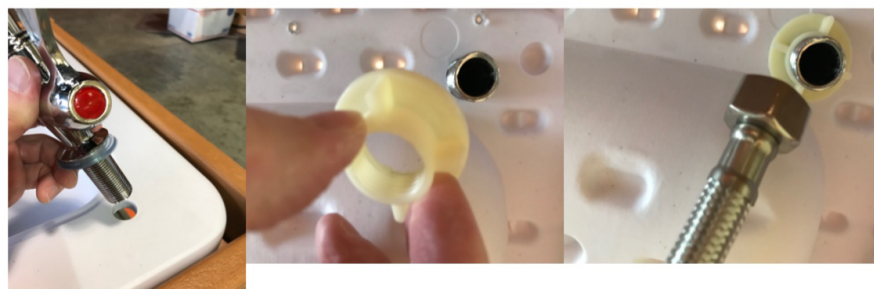
Faucet Assembly
