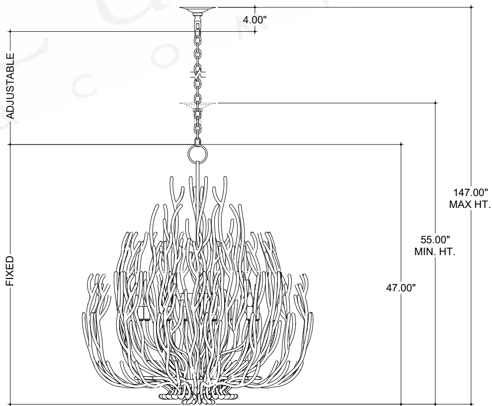
FRONT VIEW
