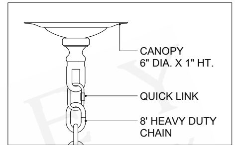
CANOPY DETAIL
