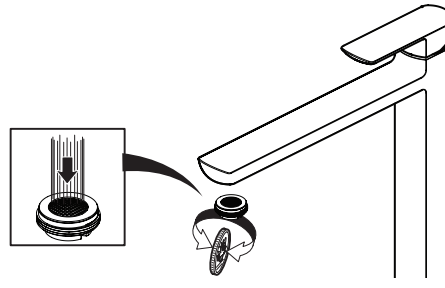
BF1291
