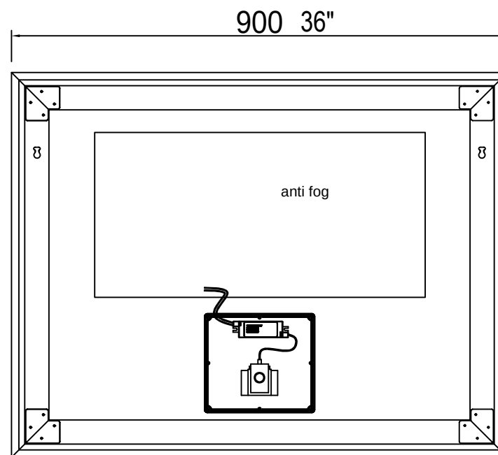
Back View
