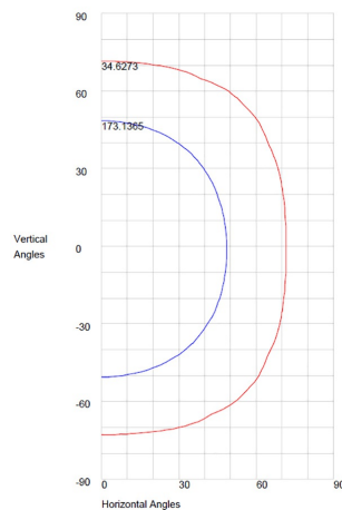
ISOCANDELA CURVES
