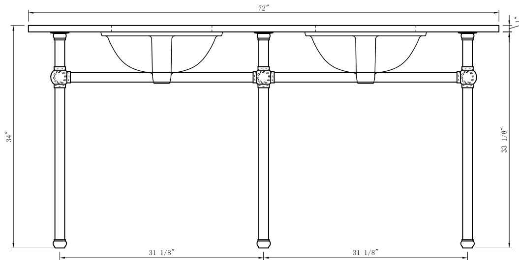
FRONT VIEW
