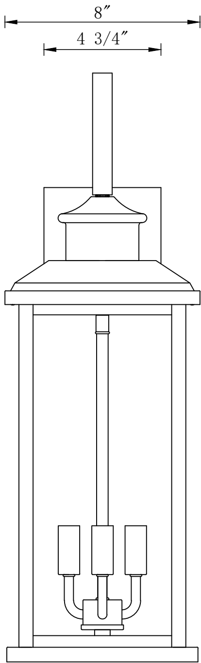
FRONT VIEW
