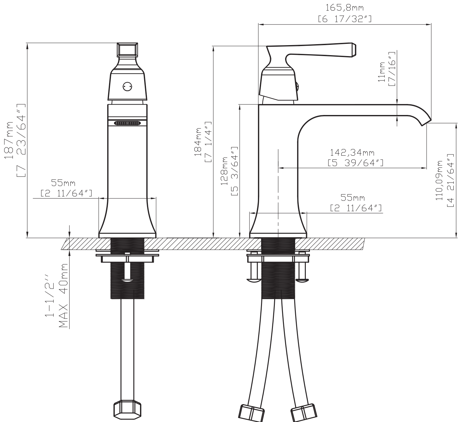
Front View
