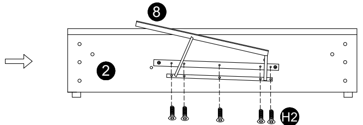
Footboard fixing holes position
