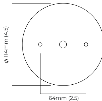
mounting plate dimensions
