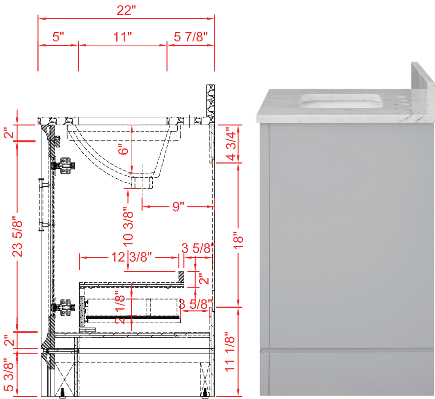
SIDE VIEW
