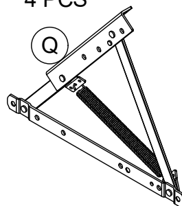
Left Support Rod 1 PC
