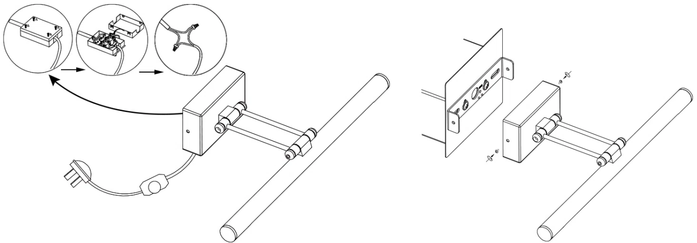
Fig.2. Hardwire Mount
