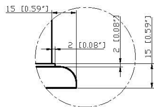
A DETAIL 4:1
