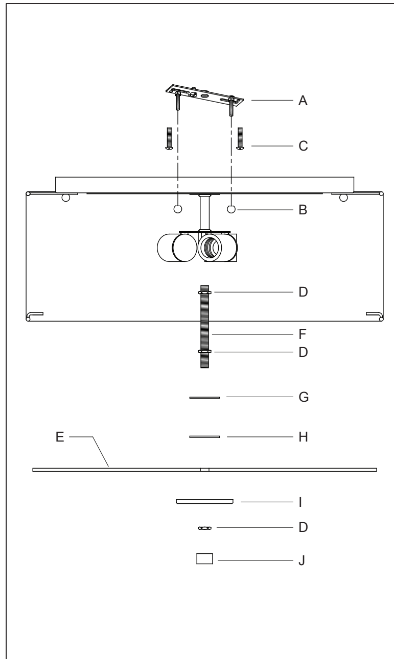
(F)Nipple
