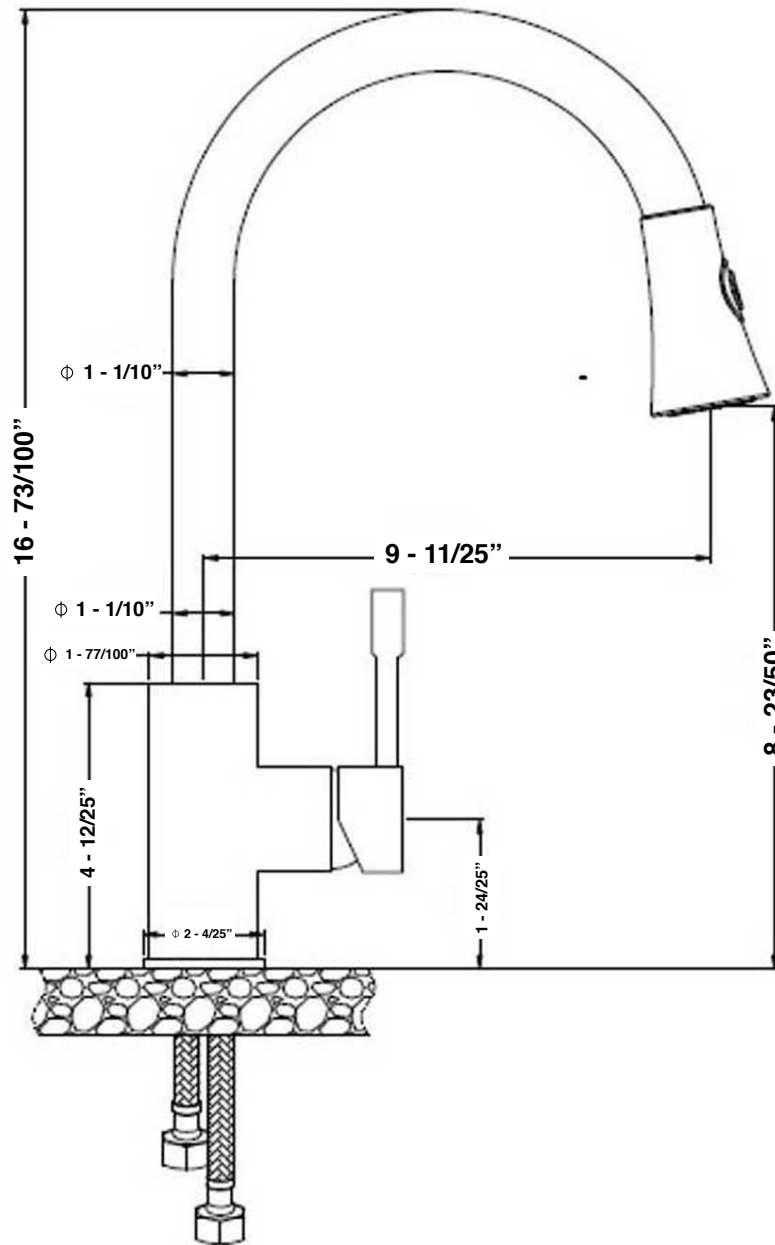
SIDE VIEW
