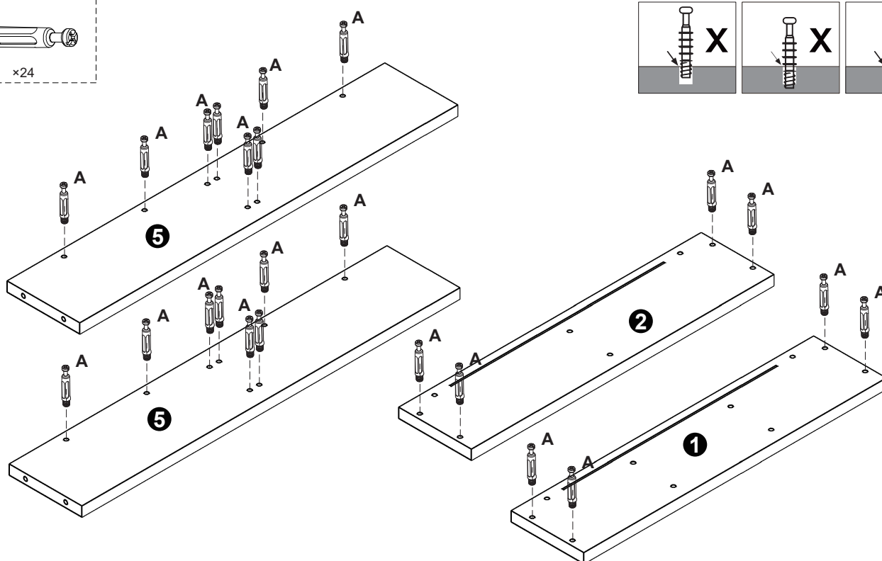
Installation method of three in one rod
