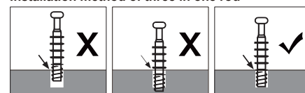
Installation method of three in one rod
