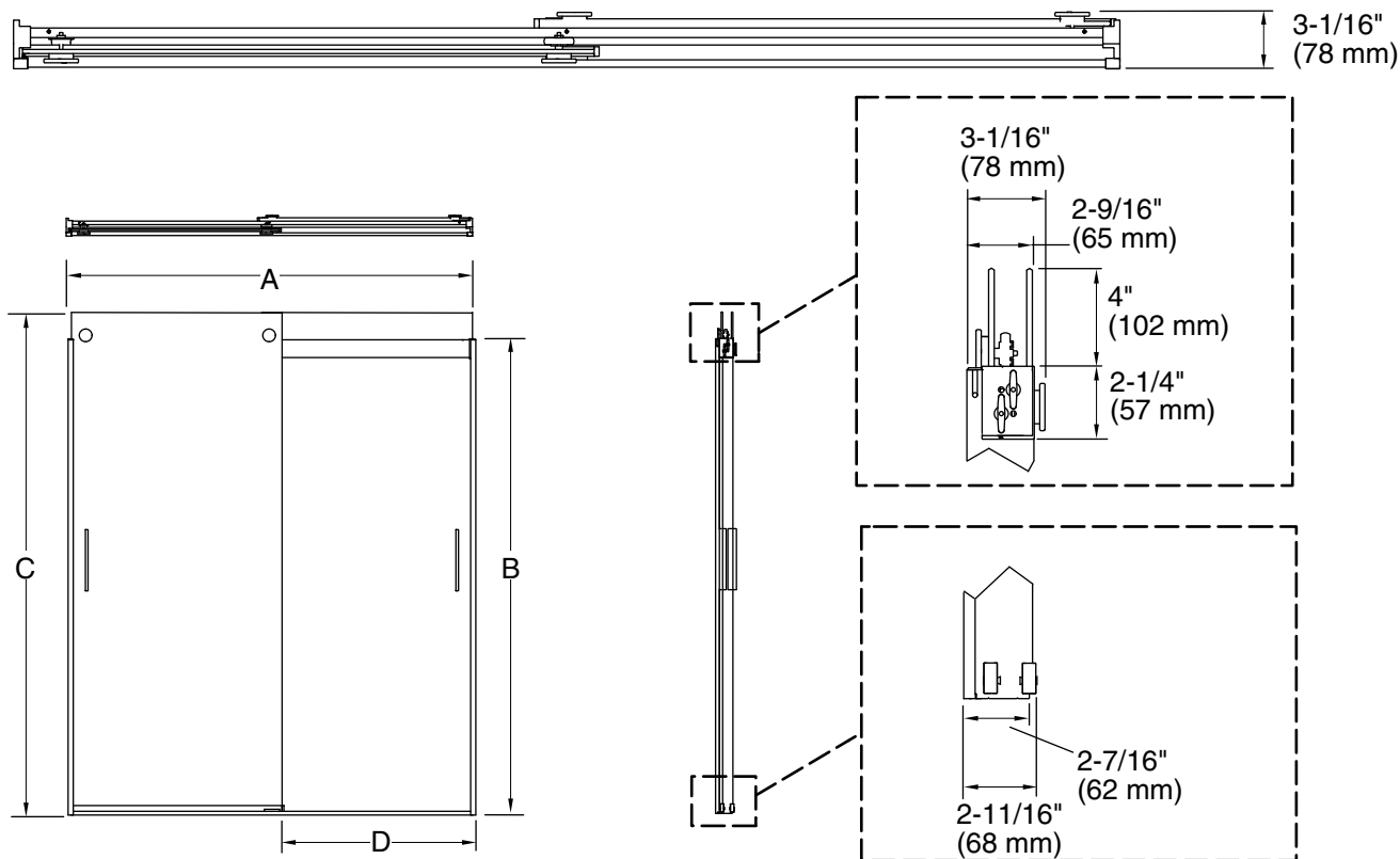
Product Diagram
