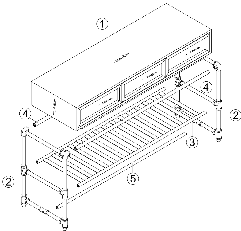
Exploded View
