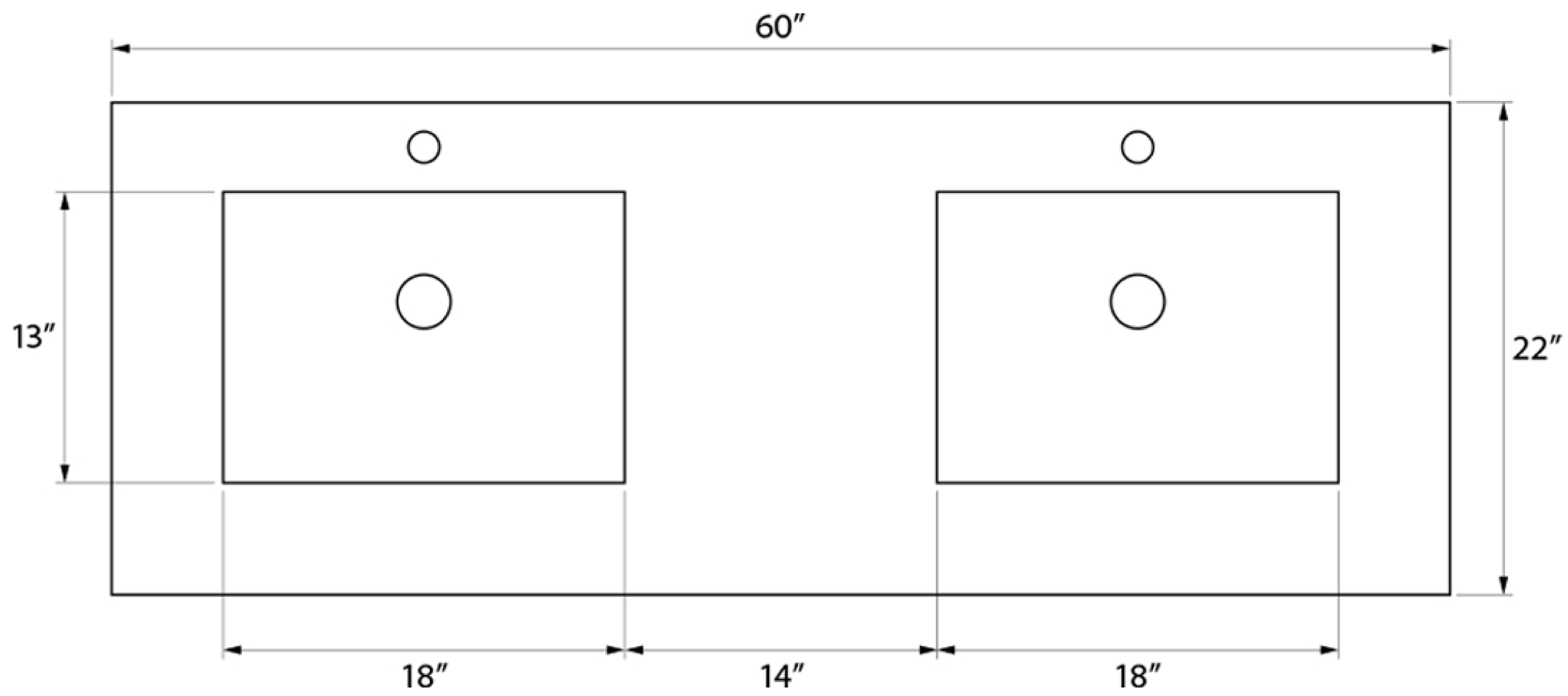
Top View
