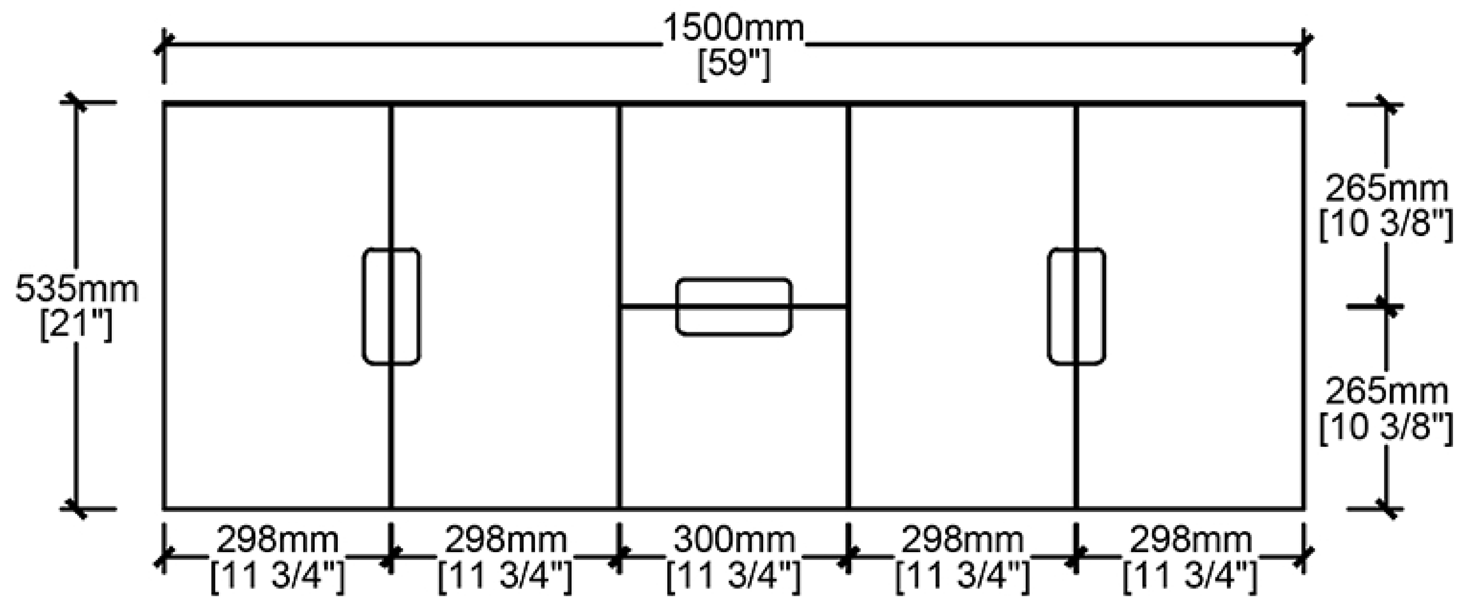
Front View
