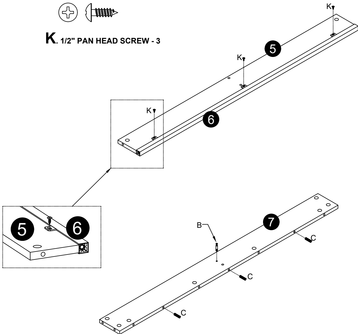
B.CAM SCREW - 1
