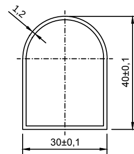
PROFILE DETAIL
