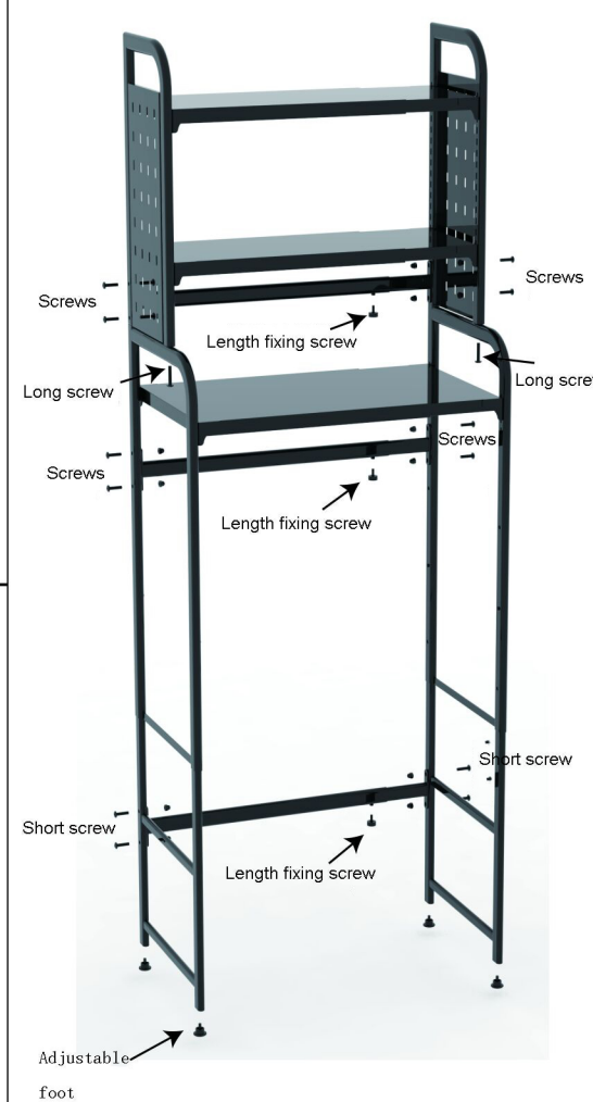
Screw position
