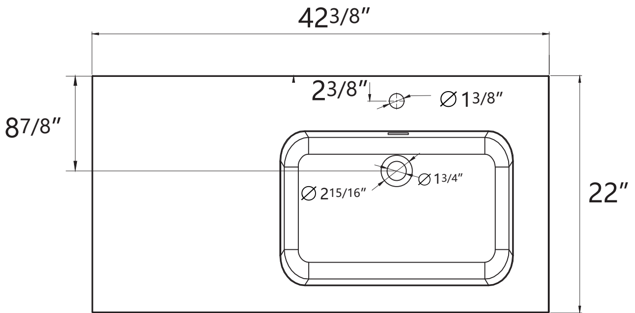
Top View
