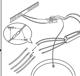
⑦ Connecting the wires into the wall electric wire.
