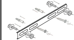
③ Filling the hole with plugs and fixing the mounting plate by screws
